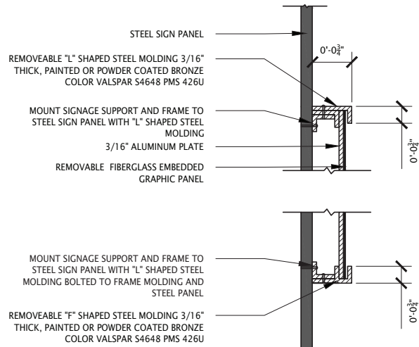
Figure ___ - Frame cross section (side)
