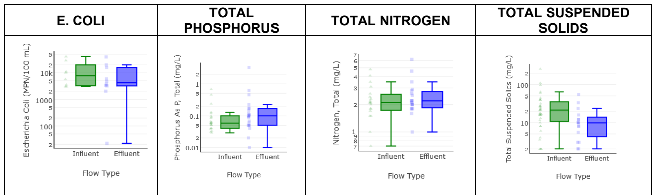
Results of swale monitoring in California for total phosphorus and total suspended solids. Total nitrogen monitoring from Texas. E coli monitoring from Oregon.
