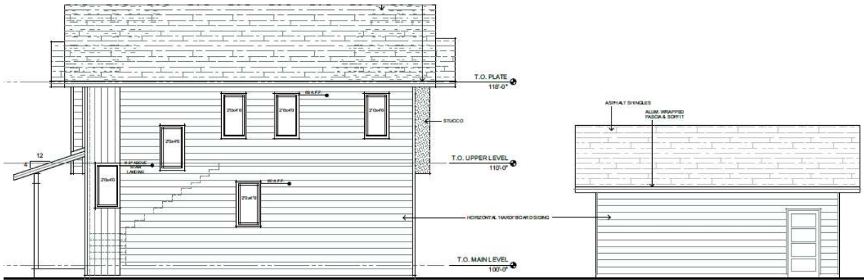
NORTH ELEVATION
